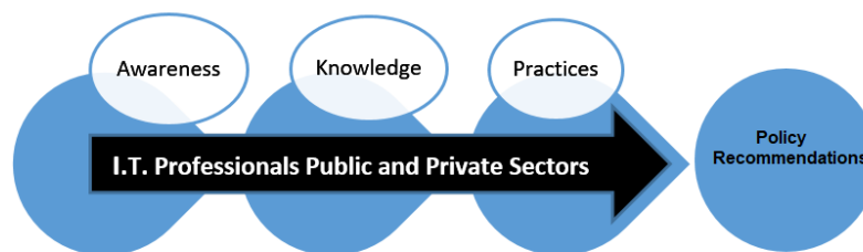
Fig. 1. Conceptual Framework
