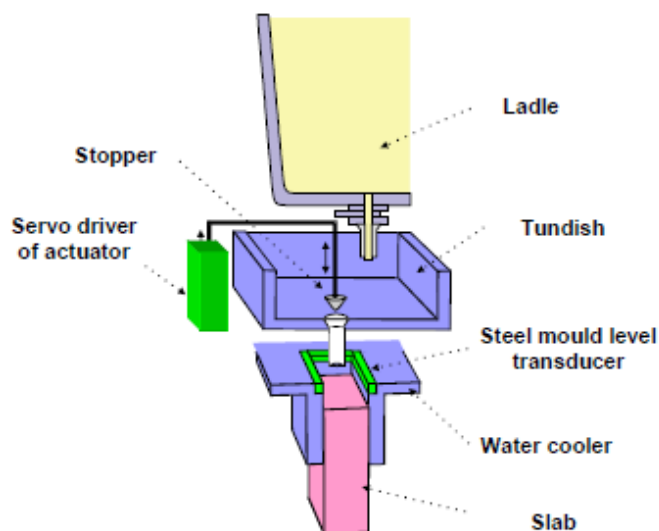
Fig. 1. Technological scheme of mould steel level control
